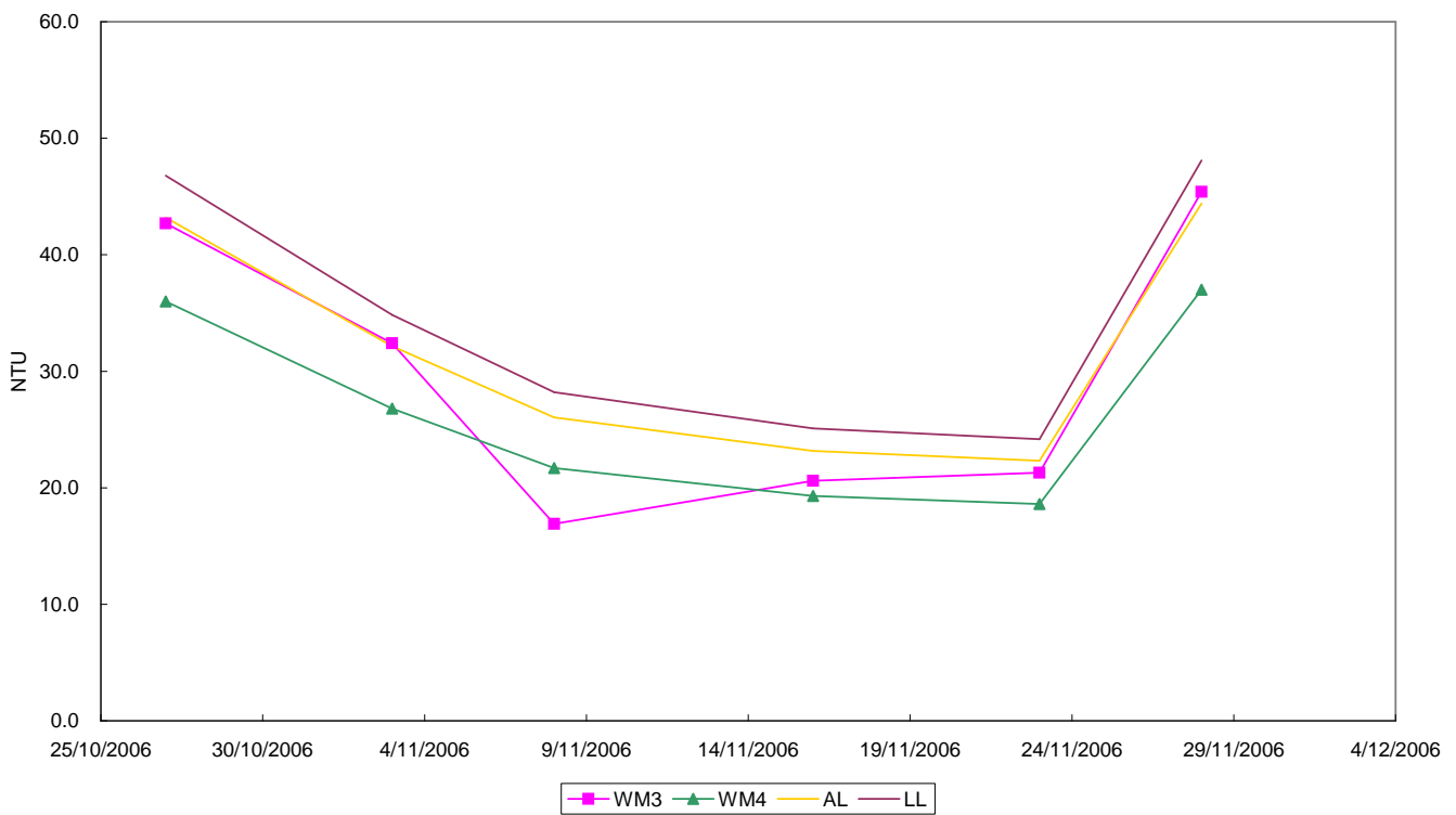
Figure 5.3f - Graphical Plot of Turbidity for WM3 & WM4
