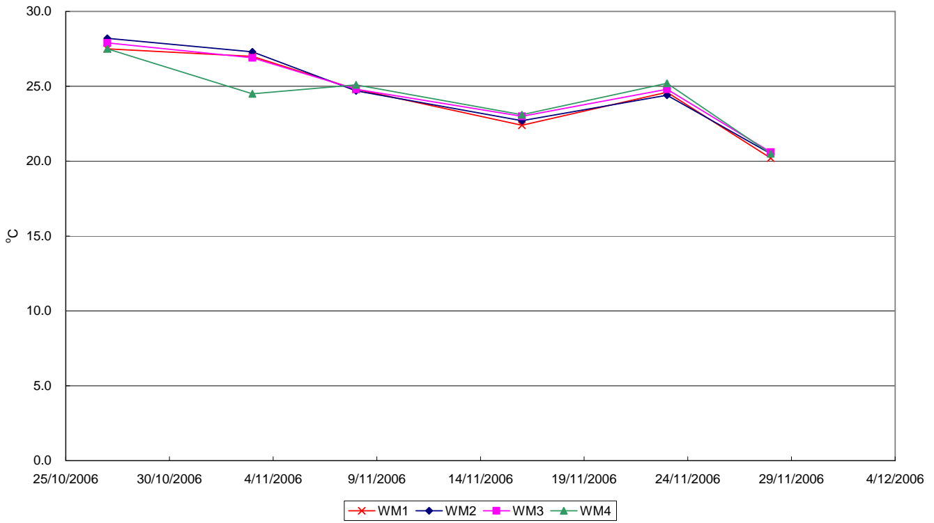
Figure 5.3a - Graphical Plot of Temperature
